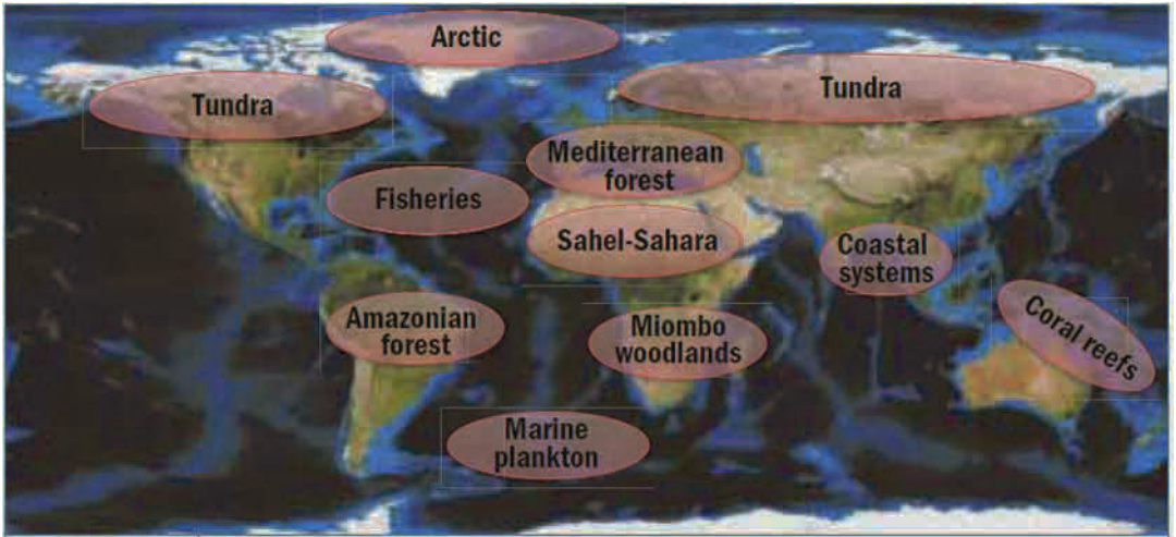
Figure 5.4. Global hotspot regions with risks of tipping points
