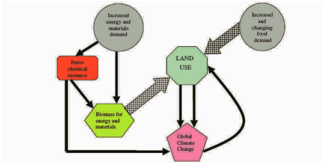
Figure 5.2. The new competition for land use: interactions and feedbacks
