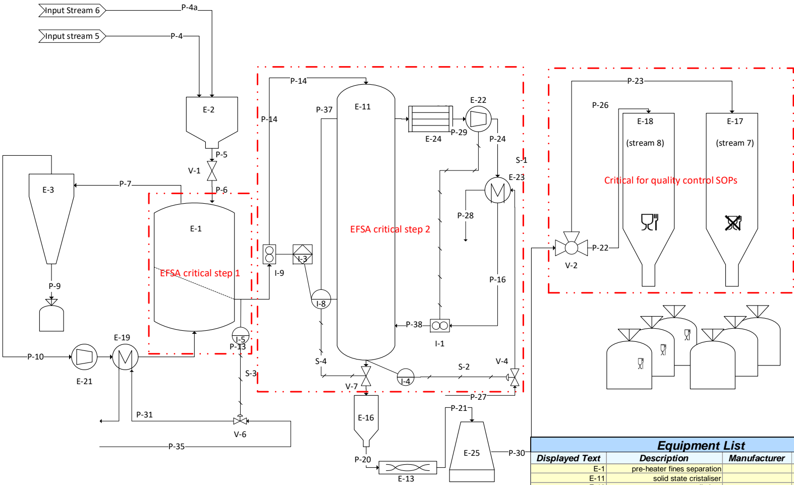
Figure 4: Piping and Instrumentation diagram of the decontamination installation. The steps/operations deemed critical by EFSA are marked with a red box
